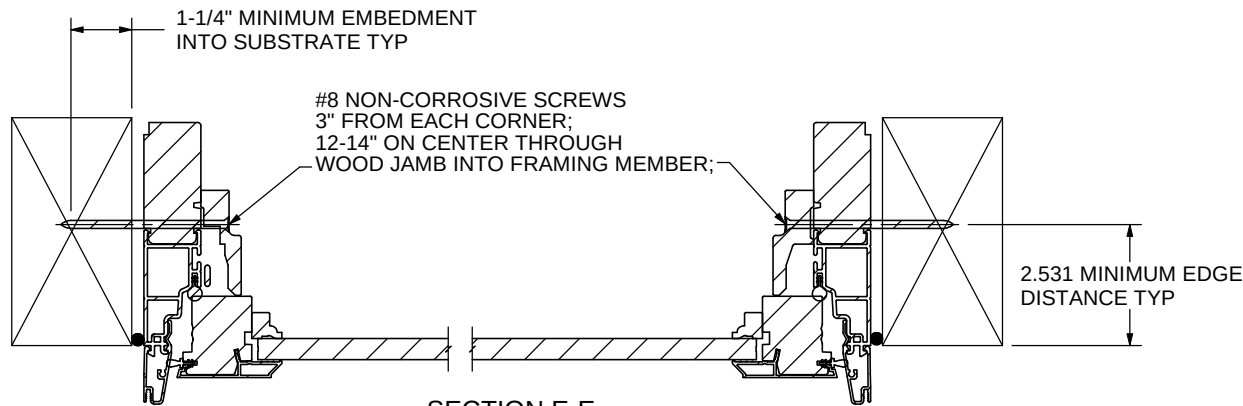
SECTION E-E SCALE 1 : 4
