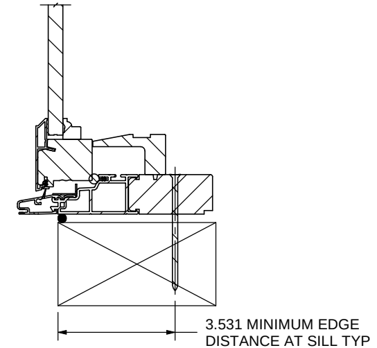
SECTION F-F SCALE 1 : 4
